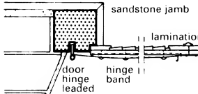
house door, old condition (horizontal section)
